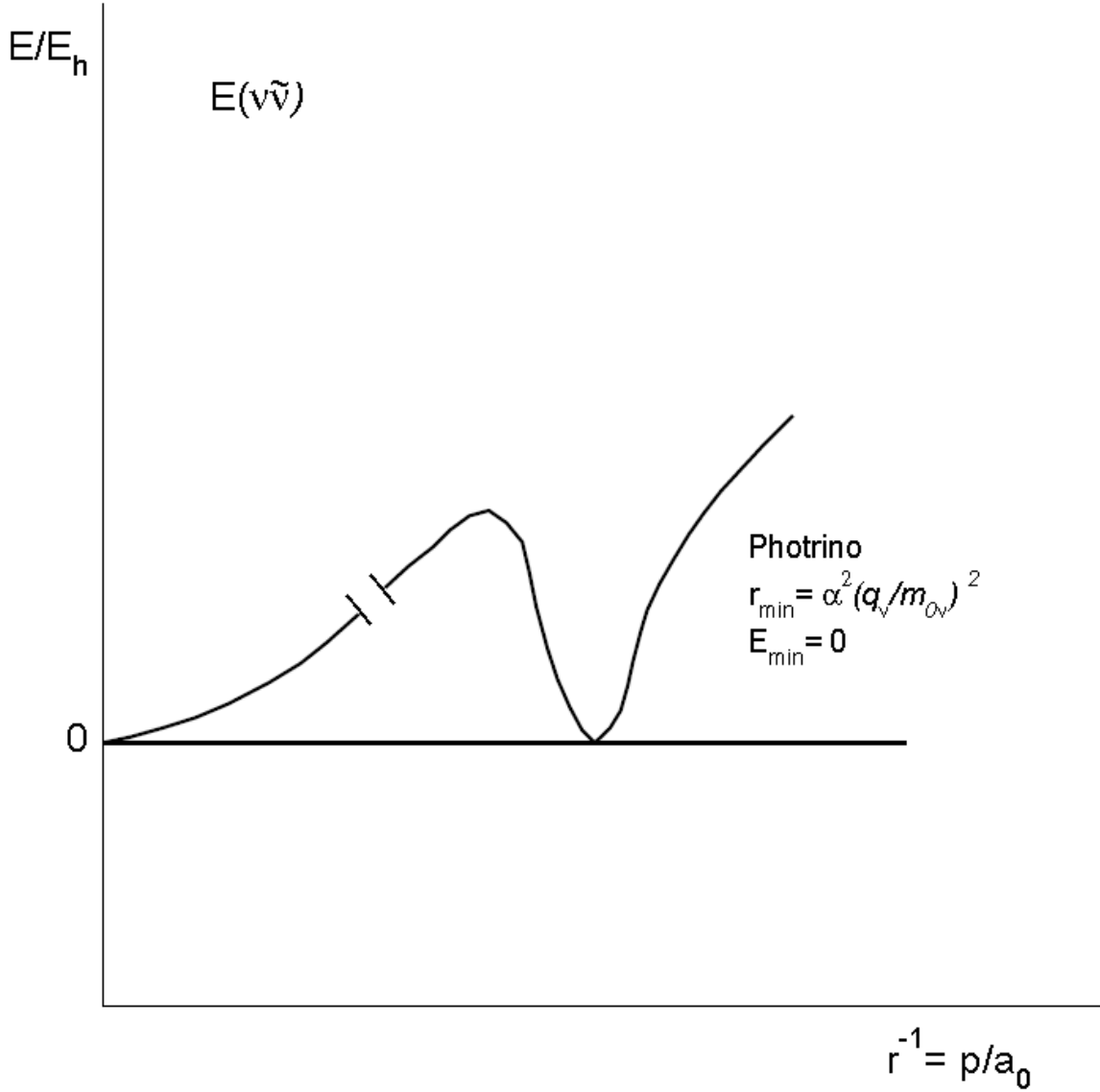
FIG. 1. Schematic diagram showing the proposed variation of the \nu\bar{\nu} system's internal energy as a function of the reciprocal of the distance between the two constituent particles. Only one minimum is expected, in contrast to the e^+e^- case shown in Fig. 1 of Ref. [7], at which point the total energy vanishes exactly, i.e. corresponding to a binding energy of 2m_{0\nu}/c^2 for the tightly bound \nu\bar{\nu} (photrino) system.
